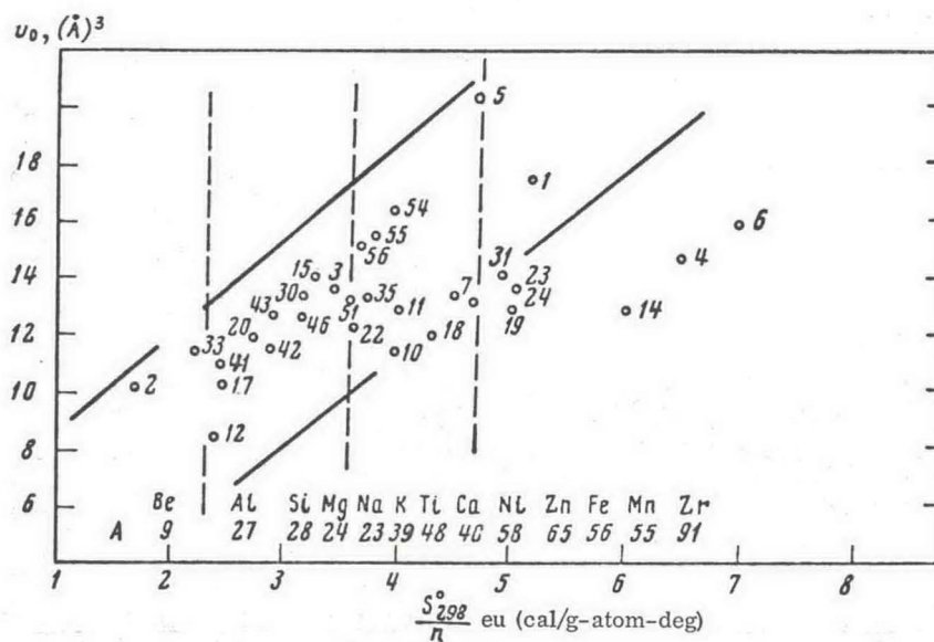
Fig. 3. \bar{S}_{298}^{\circ} (mean standard entropy) in relation to v_0 . The numbers are those of the minerals in Table 1.
