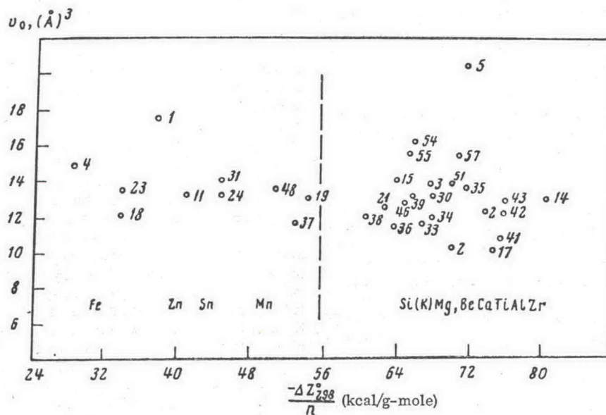
Fig. 4. Mean Gibbs free energy -\Delta Z_{298}^{\circ}/n in relation to v_0 . The numbers are those of the minerals in Table 1.
